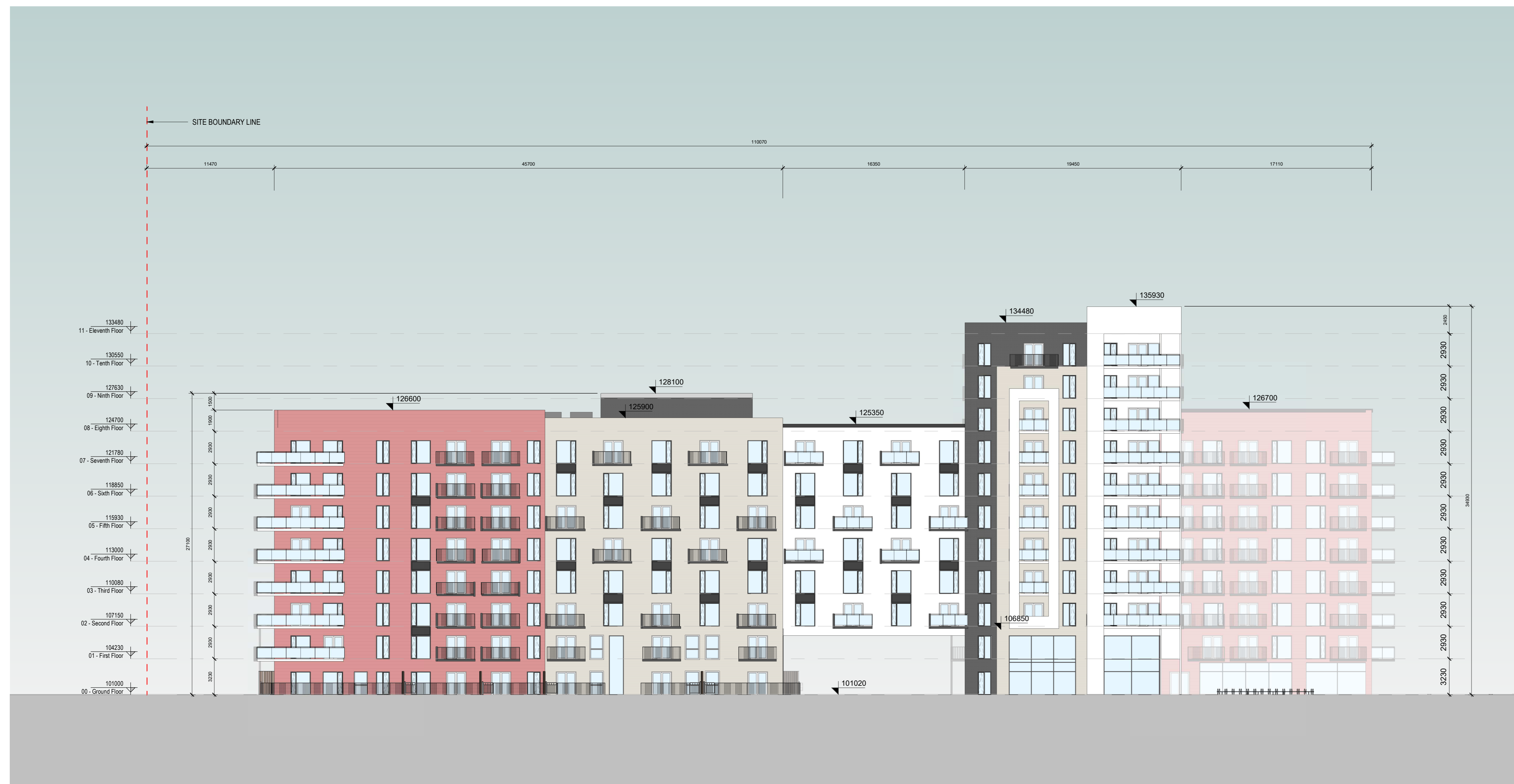
B2 Block B - Elevation B2 1:200
